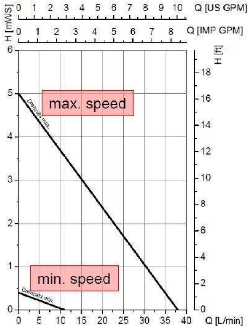
FBM-B 3100 with pump FP 314 PP 25/19-700
