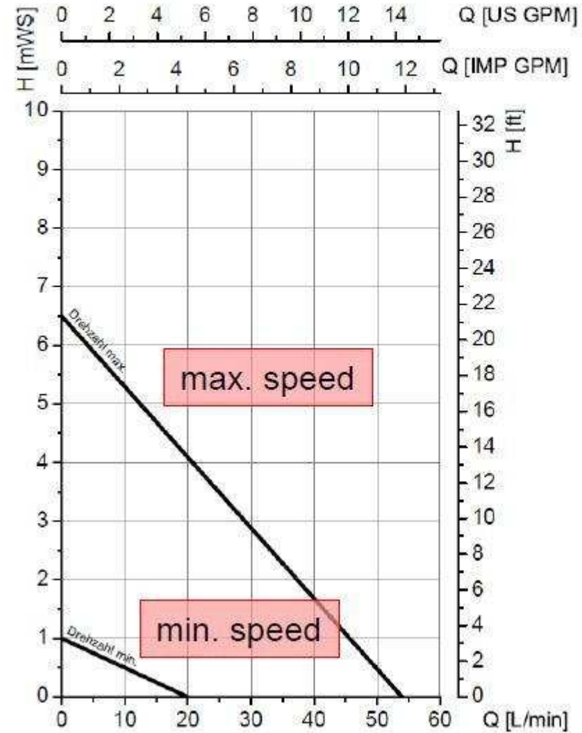
FBM-B 3100 with pump FP 314 PP 32/25-700
